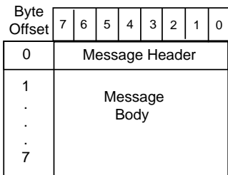
Non-Fragmented Explicit Data Field Format
